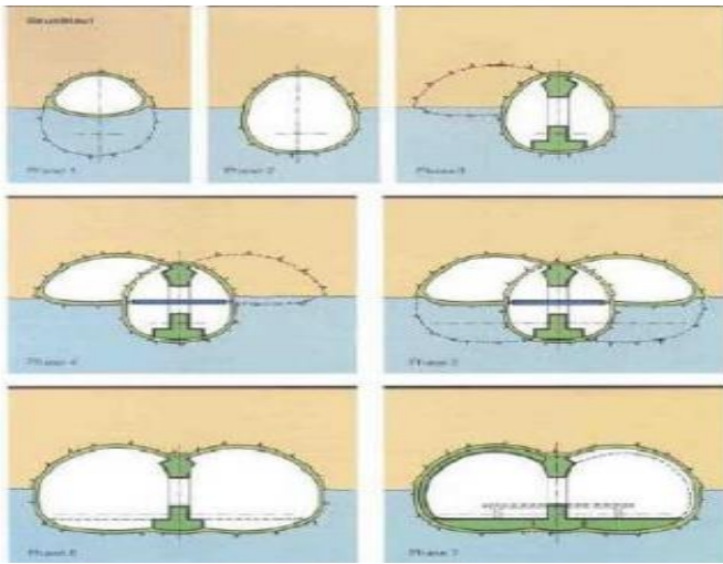
Figure:6 Basic Structure of NATM
