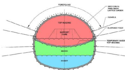
Figure:7 Cross-section Region NATM
