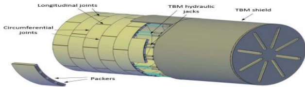
Figure:5 shows the installation of the segment linings
