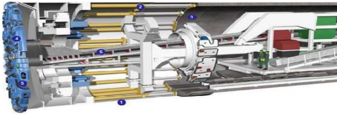
Figure:1.0 Basic Structure of TBM
