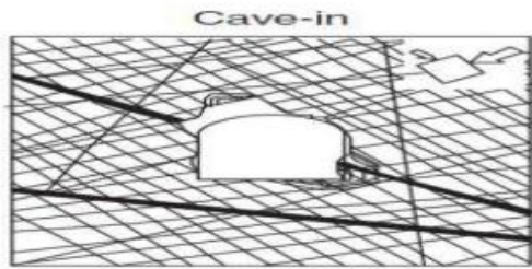
Localised brittle failure of intact rock and unravelling along discontinuities
