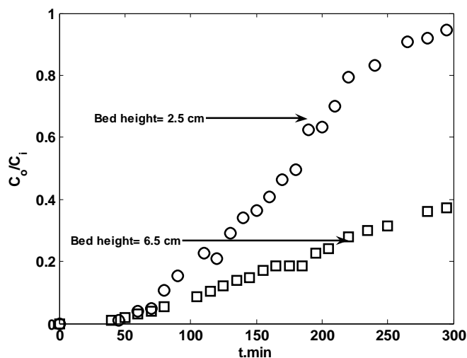
Figure 3: Effect of bed height on breakthrough curve for toluene (inlet concentration = 17000ppm, Flow rate= 60 ml/min).
