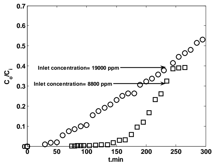
Figure 4 Effect of inlet concentration on breakthrough curve for toluene (Bed height =4.5cm Flow rate= 60ml/min)
