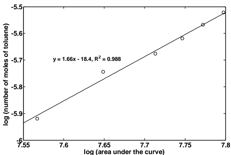
Figure 1: Calibration curve for finding the concentration of toluene vapor in a gas stream at 40° C.[7]
