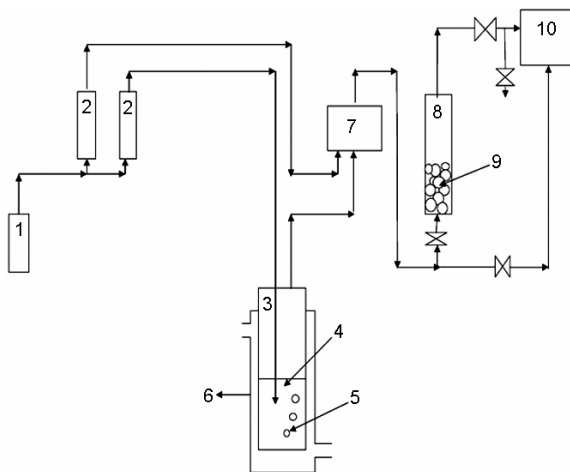
Figure. 2 Schematic diagram of the experimental set-up for xylene adsorption [1 – nitrogen gas cylinder, 2 – rotameters, 3 – VOC glass column with bubbler, 4 – liquid VOC level, 5 – gas bubbles rising through liquid VOC, 6 – jacket for maintaining isothermal conditions, 7 – mixing chamber, 8 – adsorption column, 9 – adsorbent, and 10 – gas chromatography with FID]
