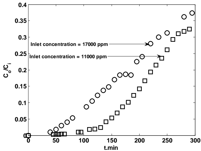
Figure 5 Effect of inlet concentration on breakthrough curve for toluene (Bed height = 6.5 cm, Flow rate=60 ml/min)
